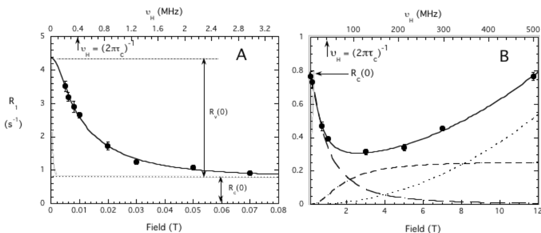
FIGURE S2. Field dependence of the ^{31}\text{P} R_1 for PMe in pure PMe SUVs at 25°C. For clarity, two magnetic field ranges are shown in the two panels with different field and relaxation rate scales: (A) low field region from 0 to 0.08 T; (B) region from 0.1 to 12 T. The upper x-axis shows the ^1\text{H} frequency scale for comparison. The lines represent best fits of (A) total dipolar R_1 = R_{dv} + R_{dc} , and (B) R_{dc} + C_L \omega_P^2 J(\tau_c, \omega_P) + C_H \omega_P^2 J(\tau_h, \omega_P) . Arrows indicate R(0) in each region as R_1 is extrapolated to zero field. Arrows on the upper ^1\text{H} frequency scale indicate how \tau_v and \tau_c can be visually estimated from the approximate half-point of the R_1 dispersion. In (B), the fitted relaxation contributions from the last three terms of Eq. 3 are shown, as a long-dashed curve for the second (dipolar) term, and a short dashed curve, and a dotted curve, for the two last (CSA) terms respectively.
