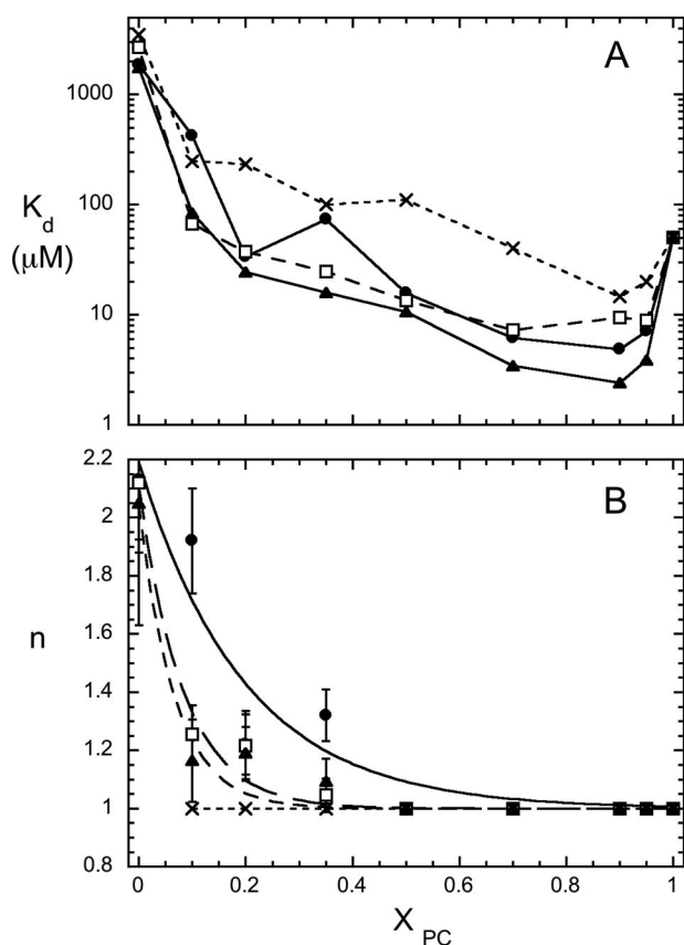
FIGURE 3. Dependence of the PI-PLC binding to mixed anionic phospholipid/PC SUVs on X_{\text{PC}} . Variation of K_d with X_{\text{PC}} (A) and variation of the cooperativity coefficient, n , with X_{\text{PC}} (B). The SUVs contained PC along with either PMe (●), PG (▲), PA (□) or PS (×).
