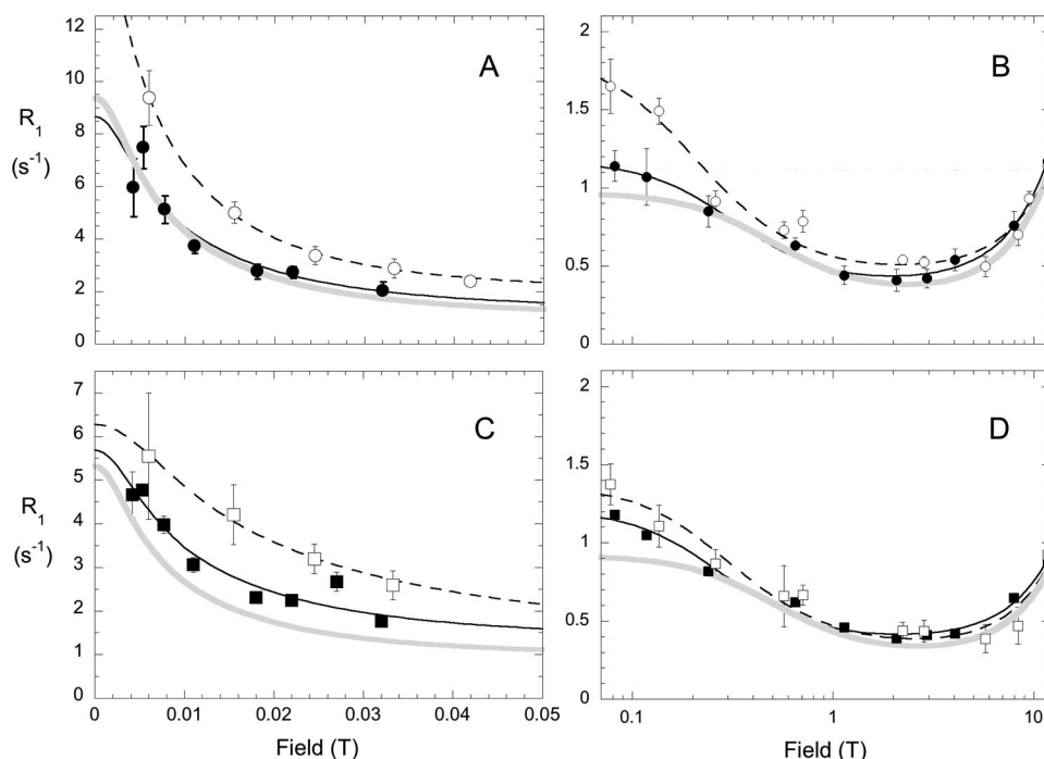
FIGURE 4. Field dependence of R_1 for PC and PMe in mixed SUVs with X_{\text{PC}} = 0.20 (filled symbols) or X_{\text{PC}} = 0.80 (open symbols) and 3 mg/ml (86 \mu\text{M} ) PI-PLC. A, field dependence of the PC R_1 from 0 to 0.05 T. B, PC R_1 from 0.07 to 11.7 T. The field dependence of the PMe R_1 is shown from 0 to 0.05 T (C) and from 0.07 to 11.7 T (D). The curves through these points represent the best fits to the simple model for R_1 dependence on field with two correlation times ( \tau_v from A and C and \tau_c from B and D). The profile exhibited by the phospholipid in the absence of protein is shown in each panel by the gray line.
